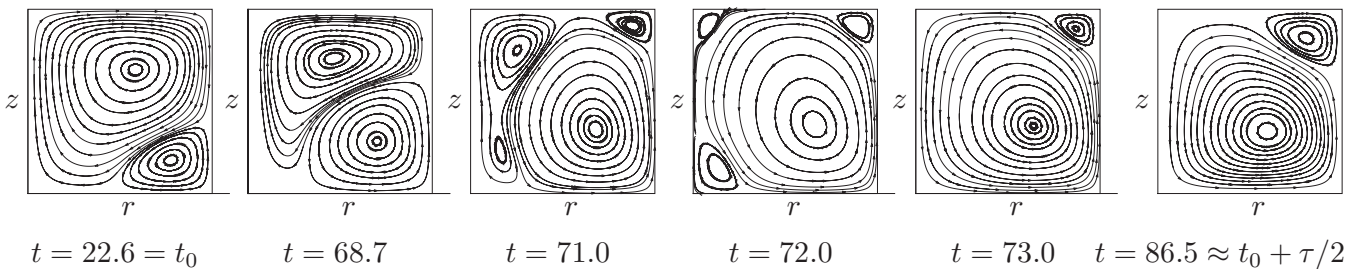
FIG. 8. Near-heteroclinic limit cycle at Ra=20\,000 , Re=63 . \Psi is shown at times indicated on time series in Fig. 9: t=22.6 ; four instants in 68 \leq t \leq 73 , during which the flow changes a great deal; and t=86.5 , approximately a half-period \tau/2 \approx 57.5 after t=22.6 . The vortex in the lower right corner grows and the vortex in the upper left corner folds and then divides into three small vortices. Two of these disappear, leaving a small vortex in the upper right corner. As in Fig. 7, the states in the second half of the cycle are related by reflection symmetry to those in the first half of the cycle and the streamfunction contours are chosen to illustrate topological features of the flow.
