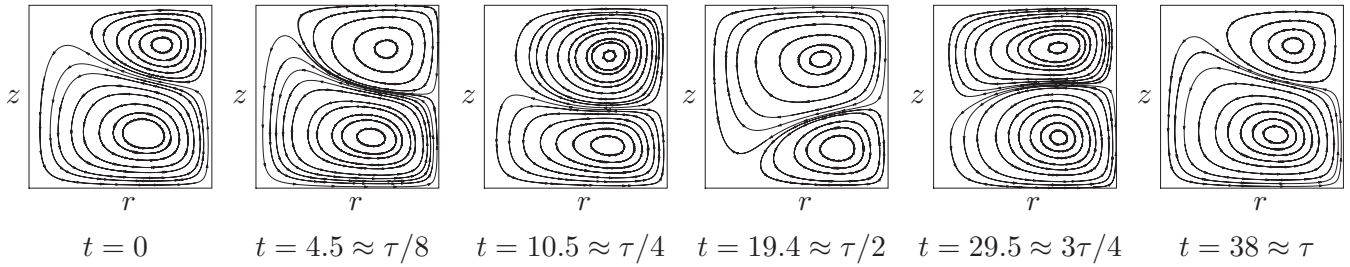
FIG. 7. Near-sinusoidal limit cycle at Ra=20\,000 , Re=110 . \Psi is shown at times near 0 , \tau/8 , \tau/4 , \tau/2 , 3\tau/4 , \tau indicated on time series in Fig. 9. Times are given in units of 1/\Omega . The overall limit cycle has reflection symmetry: the states in the second half of the cycle are related by reflection symmetry to those in the first half of the cycle. The vortex in the upper right corner is smaller during the first half of the cycle and larger during the second half. The streamfunction contours are not equally spaced, but instead chosen to illustrate topological features of the flow.
