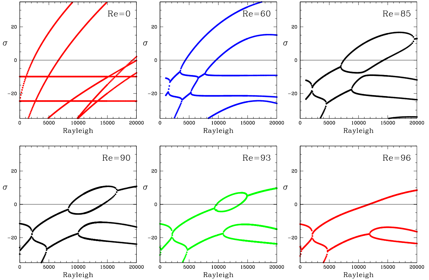
FIG. 14. (Color online) Real part \sigma of leading eigenvalues as a function of Ra for six values of Re . For Re=0 , the eigenvalues are real and cross transversely. Zero crossings at Ra=2260 and Ra=6640 correspond to pitchfork bifurcations. Purely thermal and azimuthal eigenvalues at \sigma=-9.87 and \sigma=-24.6 , respectively, are independent of Ra . When Re>0 , the transverse crossings become complex-conjugate pairs, over Ra intervals which widen with increasing Re . By Re=96 , the bifurcating eigenvalue is a complex-conjugate pair, leading to a Hopf bifurcation at Ra=11\ 856 .
